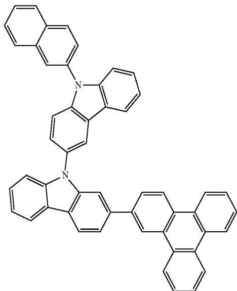
Chemical Formula 1-14
