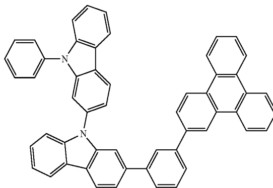
Chemical Formula 1-50
