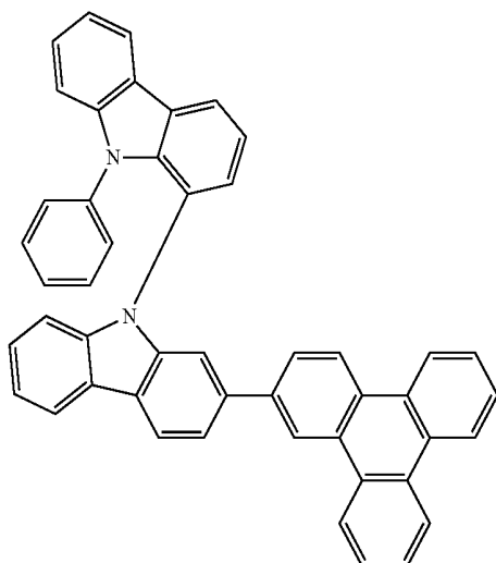
Chemical Formula 1-39
