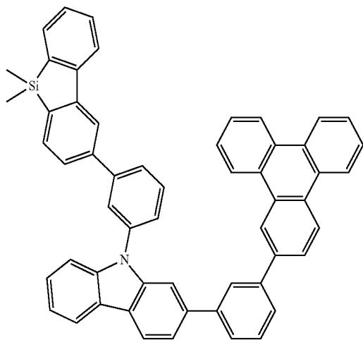
Chemical Formula 1-10
