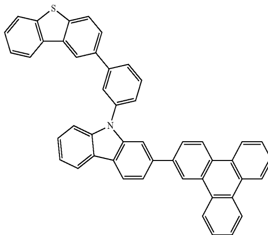
Chemical Formula 1-74
