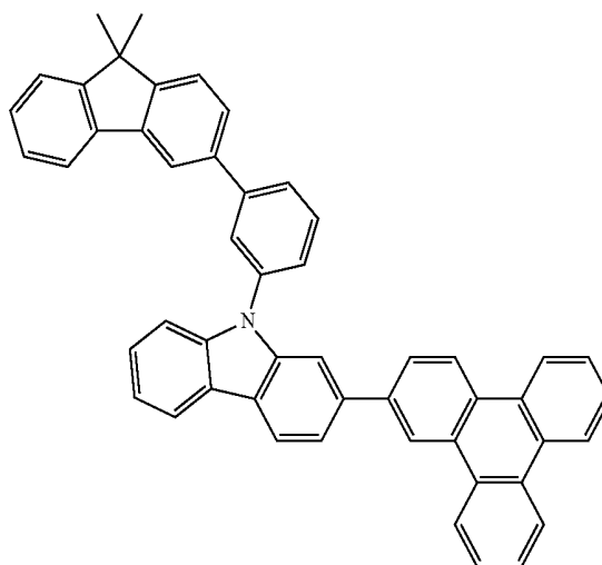
Chemical Formula 1-70
