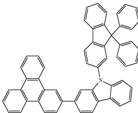
Chemical Formula 1-15
