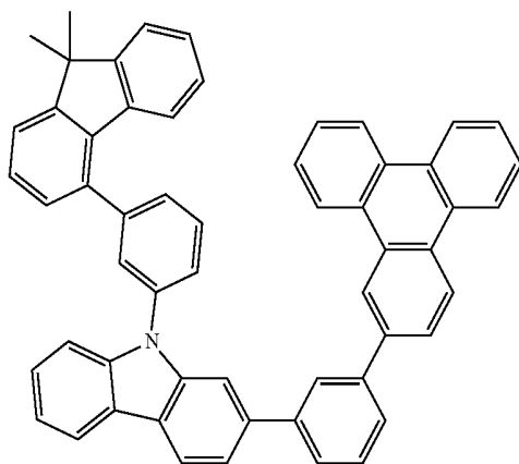
Chemical Formula 1-81
