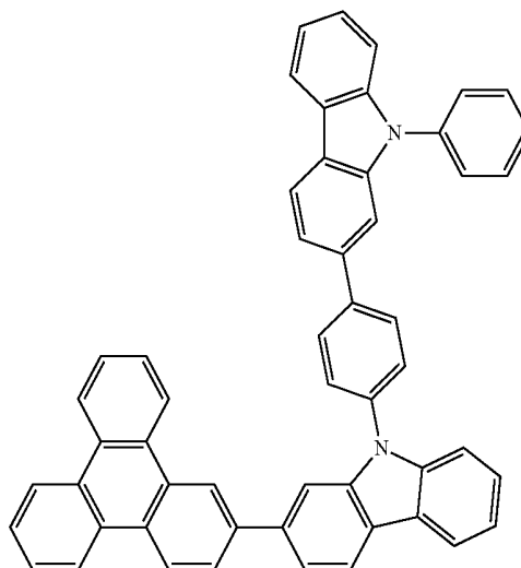
Chemical Formula 1-11
