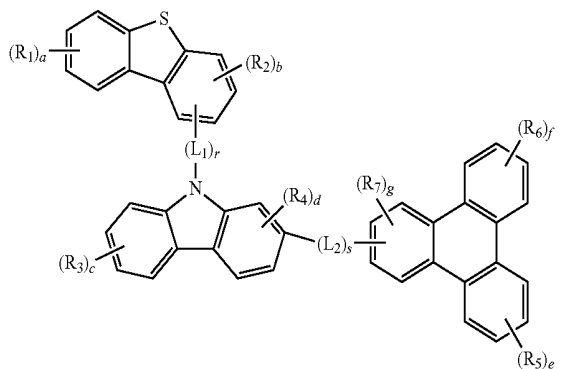
[Chemical Formula 6]
