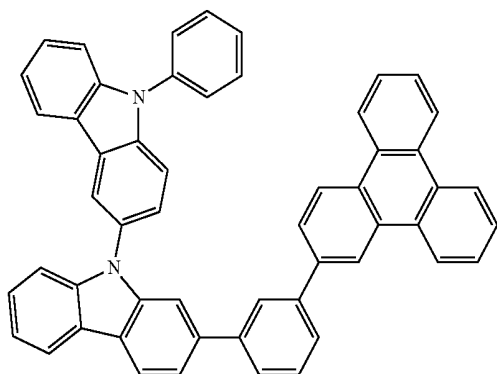
Chemical Formula 1-49
