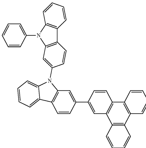
Chemical Formula 1-2
