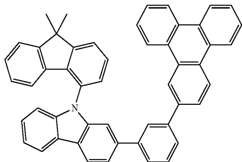
Chemical Formula 1-55
