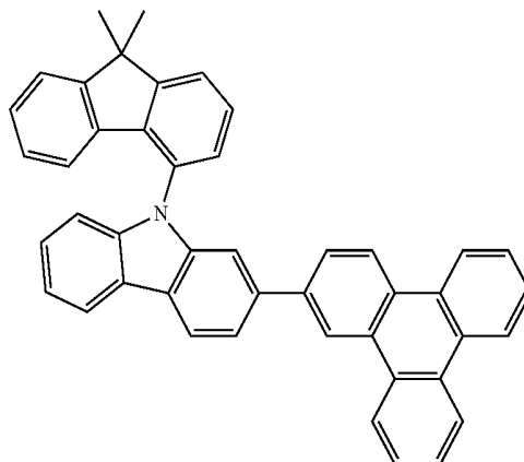
Chemical Formula 1-40
