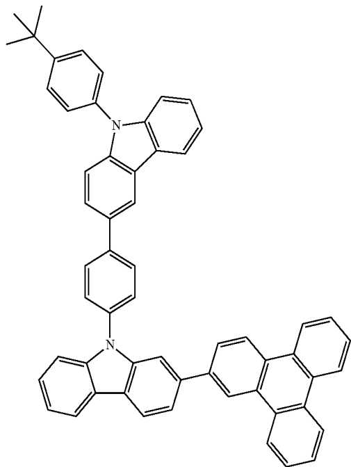
Chemical Formula 1-8
