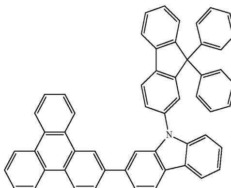
Chemical Formula 1-15
