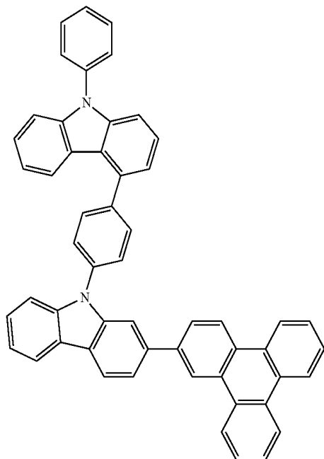
Chemical Formula 1-69
