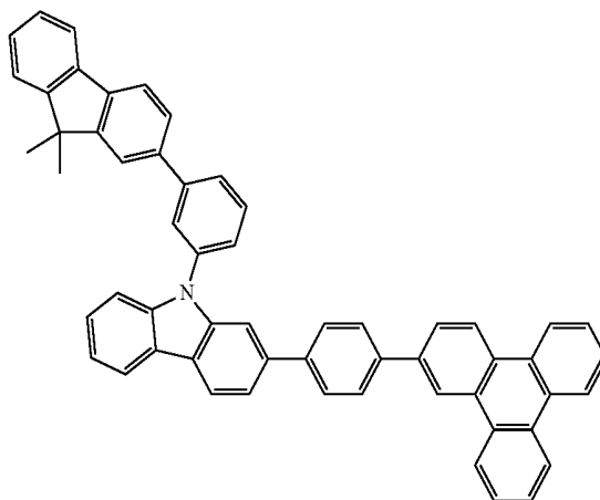
Chemical Formula 1-16
