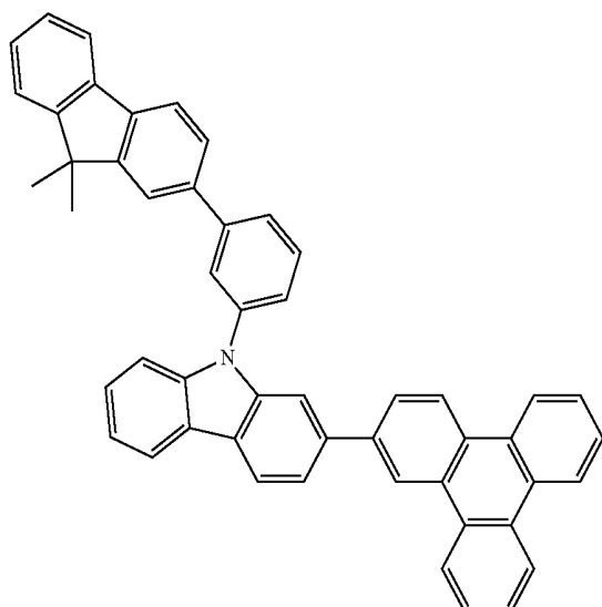
Chemical Formula 1-14
