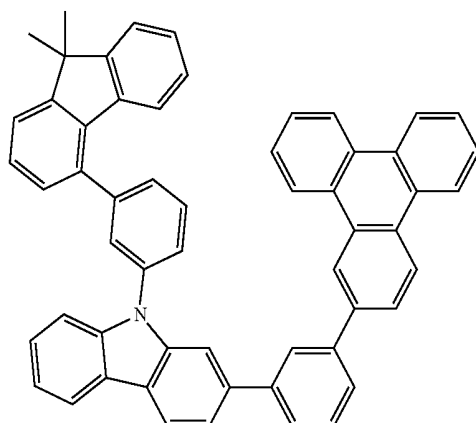
Chemical Formula 1-81
