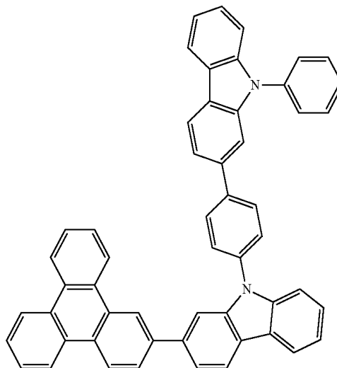
Chemical Formula 1-13
