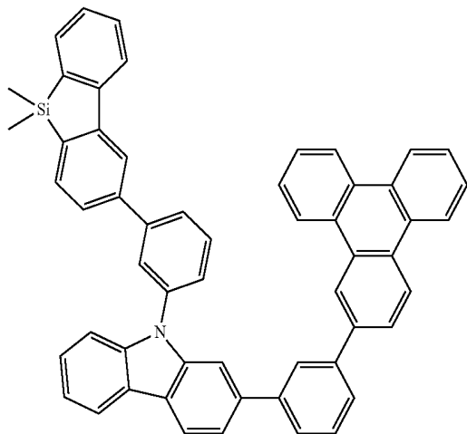
Chemical Formula 1-12
