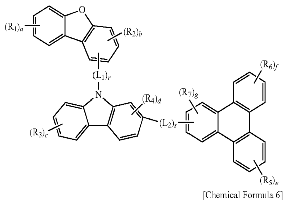
[Chemical Formula 6]
