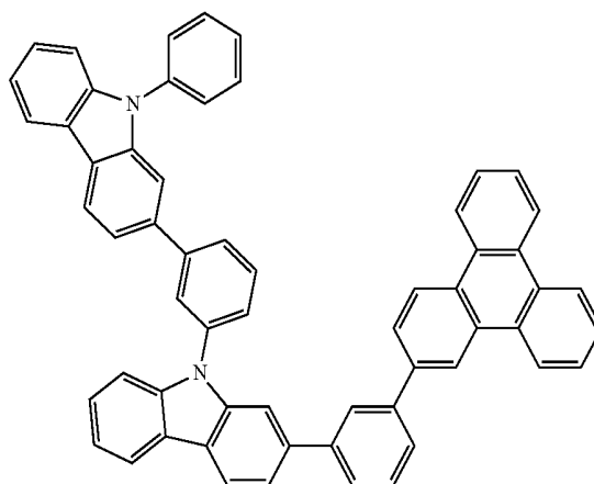
Chemical Formula 1-80
