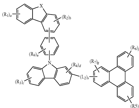
[Chemical Formula 3]
