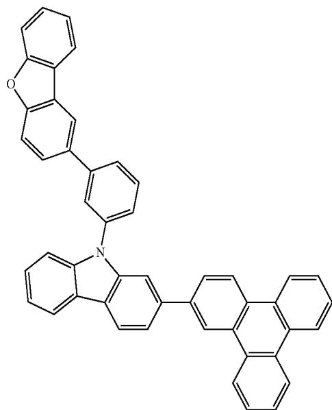
Chemical Formula 1-24
