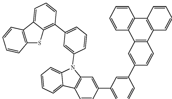
Chemical Formula 1-51
