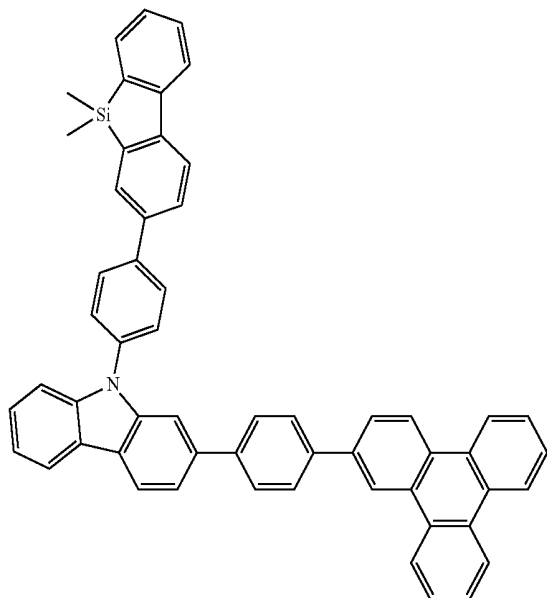
Chemical Formula 1-33
