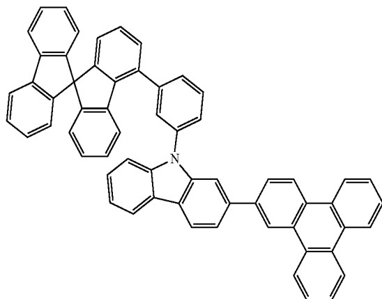
Chemical Formula 1-77
