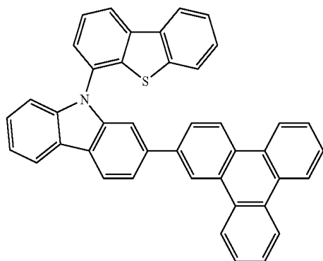
Chemical Formula 1-41
