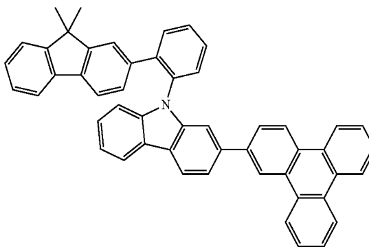
Chemical Formula 1-21
