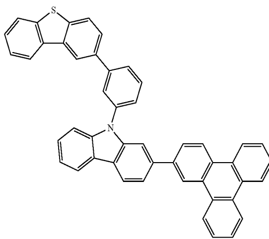
Chemical Formula 1-72
