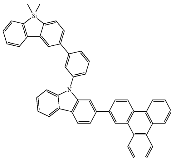
Chemical Formula 1-75
