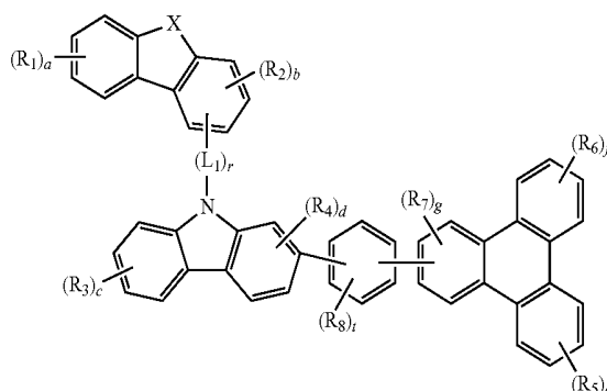
[Chemical Formula 2]
