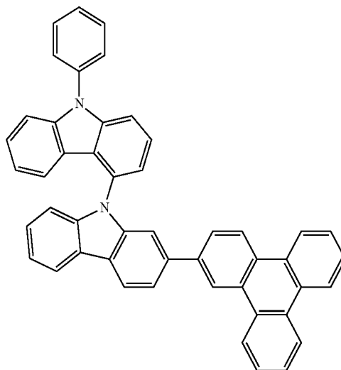
Chemical Formula 1-38
