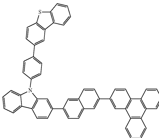
Chemical Formula 1-30
