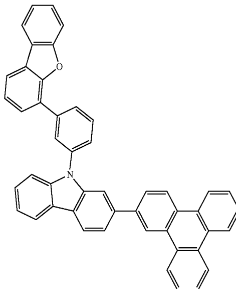
Chemical Formula 1-74
