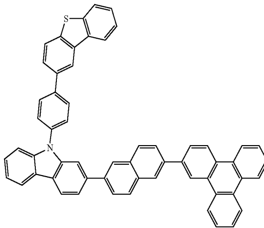
Chemical Formula 1-30
