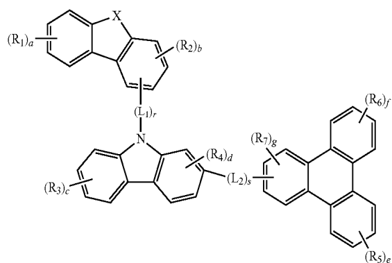
[Chemical Formula 1]
