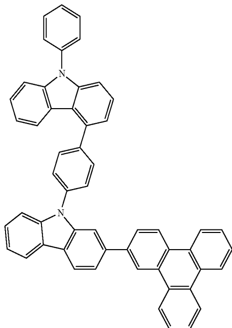
Chemical Formula 1-67
