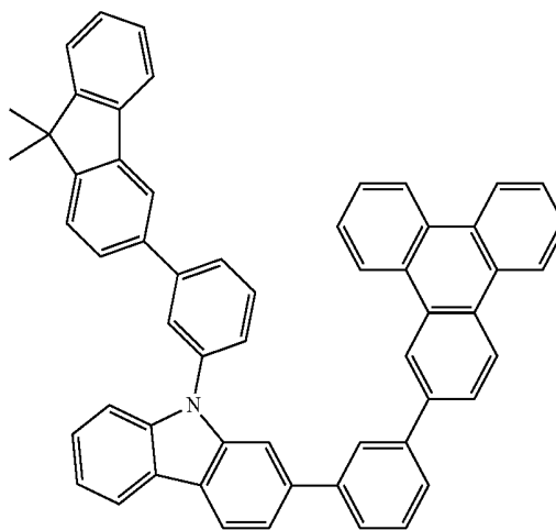
Chemical Formula 1-82
