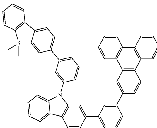
Chemical Formula 1-7
